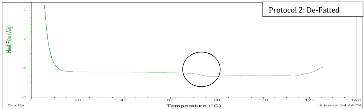
Figure 2.10 Gelatinization not seen in DSC samples without performing de-fatting procedure.
